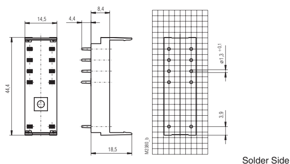
Solder Side
