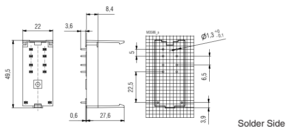
Solder Side
