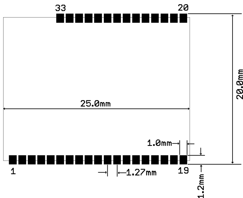
Figure 9: Recommended Footprint
