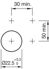
Mounting cut-outs [mm]
