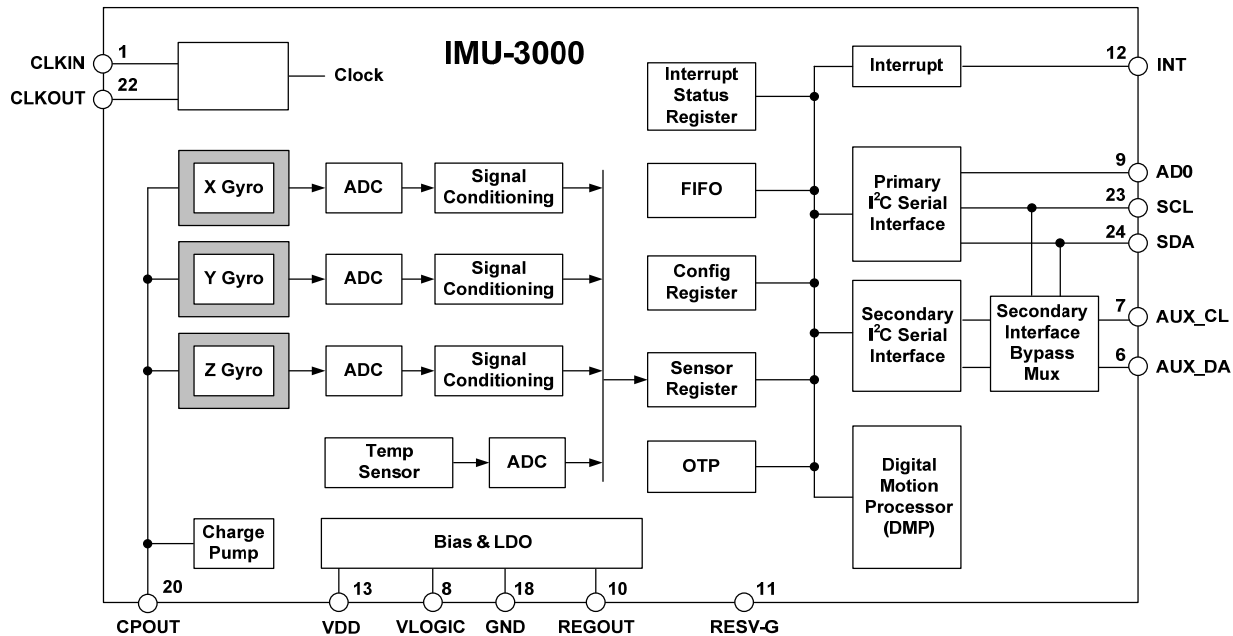
Figure 3: IMU-3000 Functional Block Diagram
