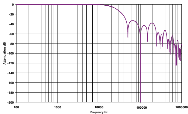
Figure 51. Digital Filter response for OS4
