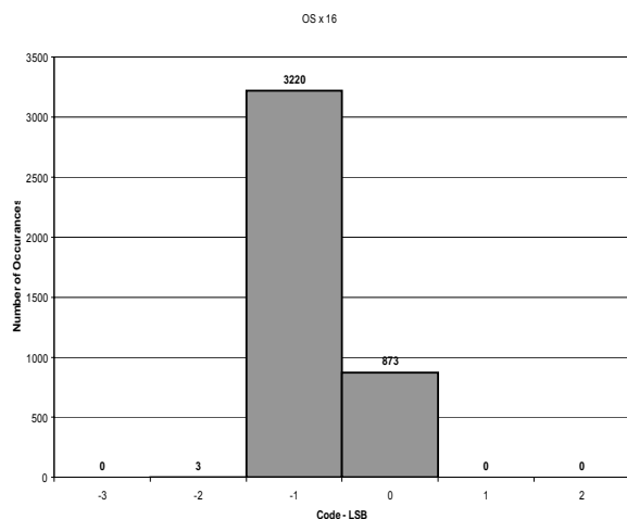
Figure 49. Histogram of codes – OS x 16 (3 codes)
