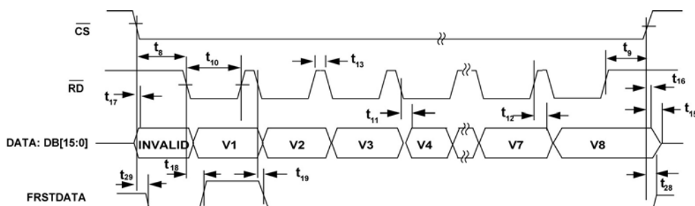
Figure 4 Parallel Mode Separate \overline{CS} and \overline{RD} pulses
