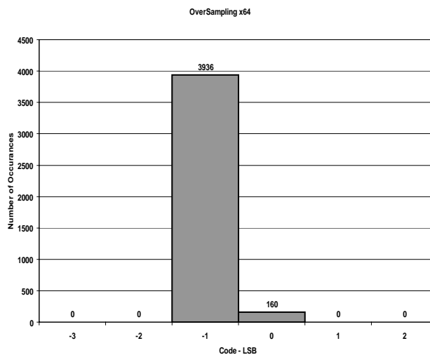
Figure 50. Histogram of codes – OS x 64 (2 codes)
