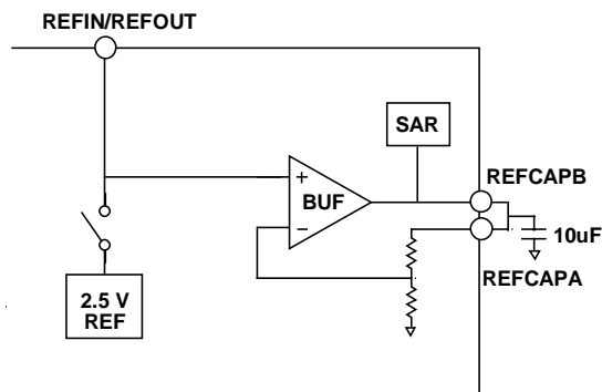
Figure 38 Reference Circuitry
