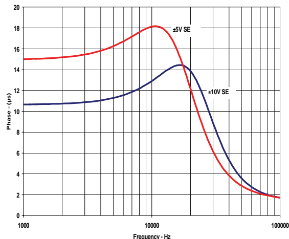
Figure 36. Analog Anti-Alias Filter Phase Response
