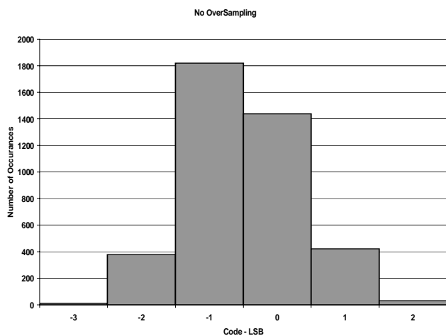
Figure 47. Histogram of codes – No OS – (6 codes)
