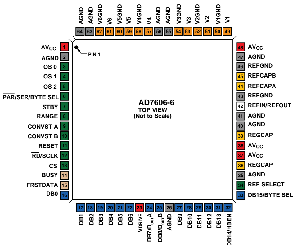
Figure 9. AD7606-6 Pin Configuration
