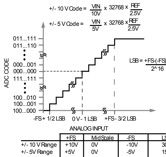
Figure 37. AD7606 Transfer Characteristic
