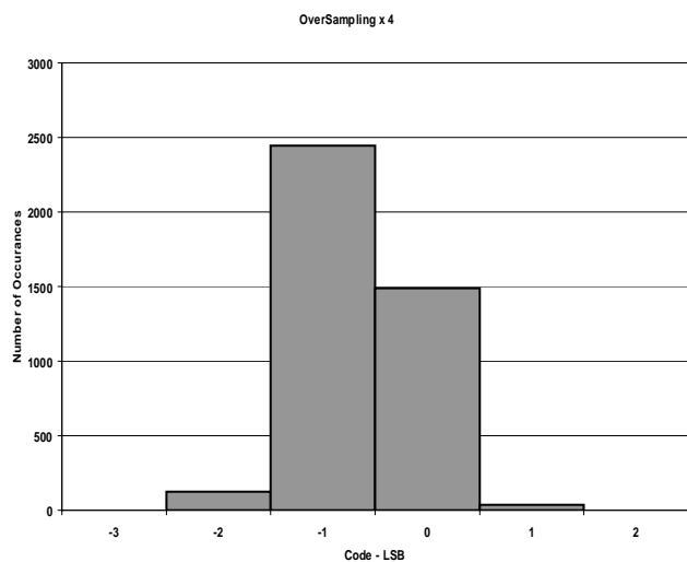
Figure 48 Histogram Of Codes – OS x 4.(4 codes)
