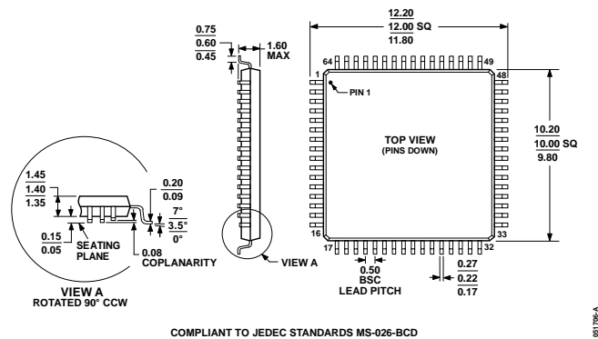
Figure 57 64-Lead Low Profile Quad Flat Package [LQFP]
