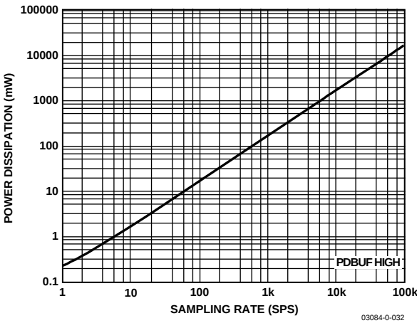
Figure 26. Power Dissipation vs. Sample Rate
