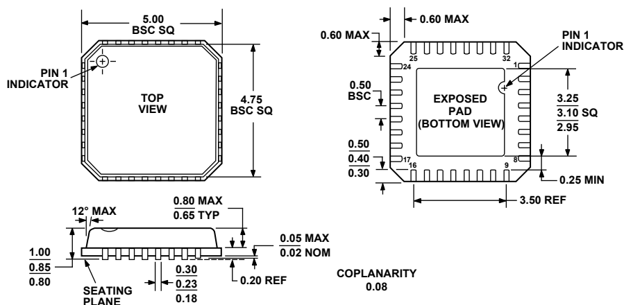
Figure 12. 32-Lead Lead Frame Chip Scale Package [LFCSP_VQ] 5 mm x 5 mm Body, Very Thin Quad (CP-32-2) Dimensions shown in millimeters
