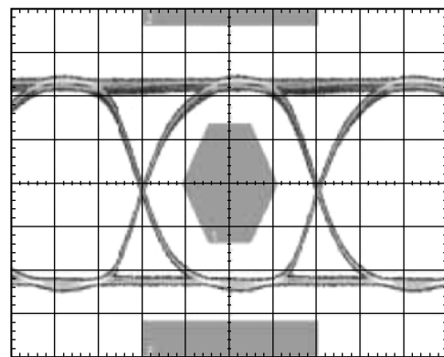
Figure 11. A 1.244 Mbps Optical Eye. Temperature at 85°C. Average Power = 0 dBm, Extinction Ratio = 10 dBm, PRBS 31 Pattern, 1 Gb Ethernet Mask. Eye Obtained Using a DFB Laser.
