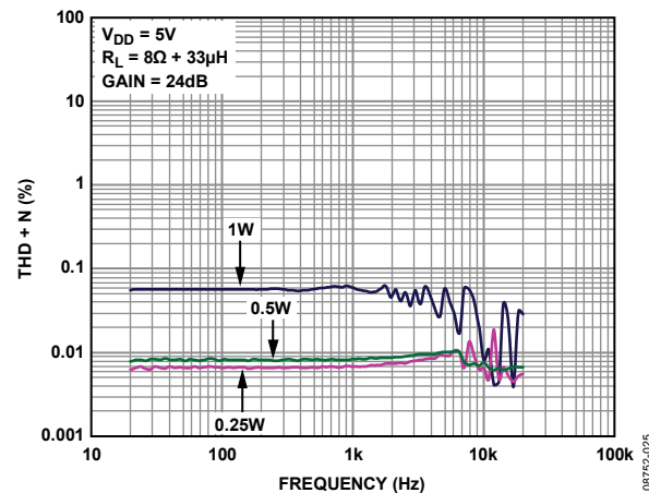
Figure 9. THD + N vs. Frequency, V DD = 5V, R L = 8 Ω, Gain = 24 dB
