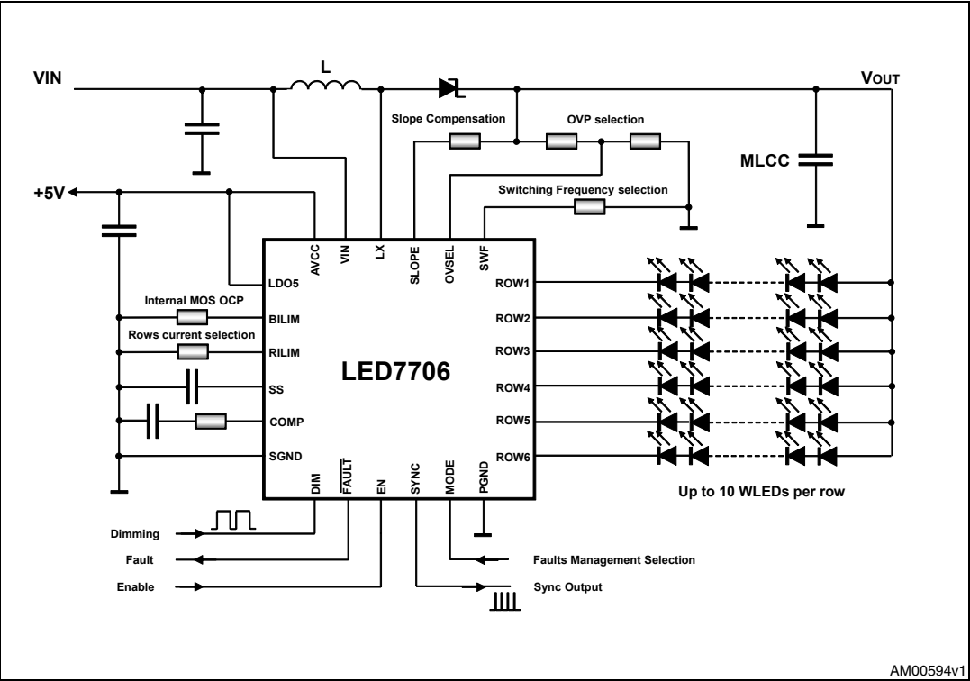
Figure 1. Application circuit
