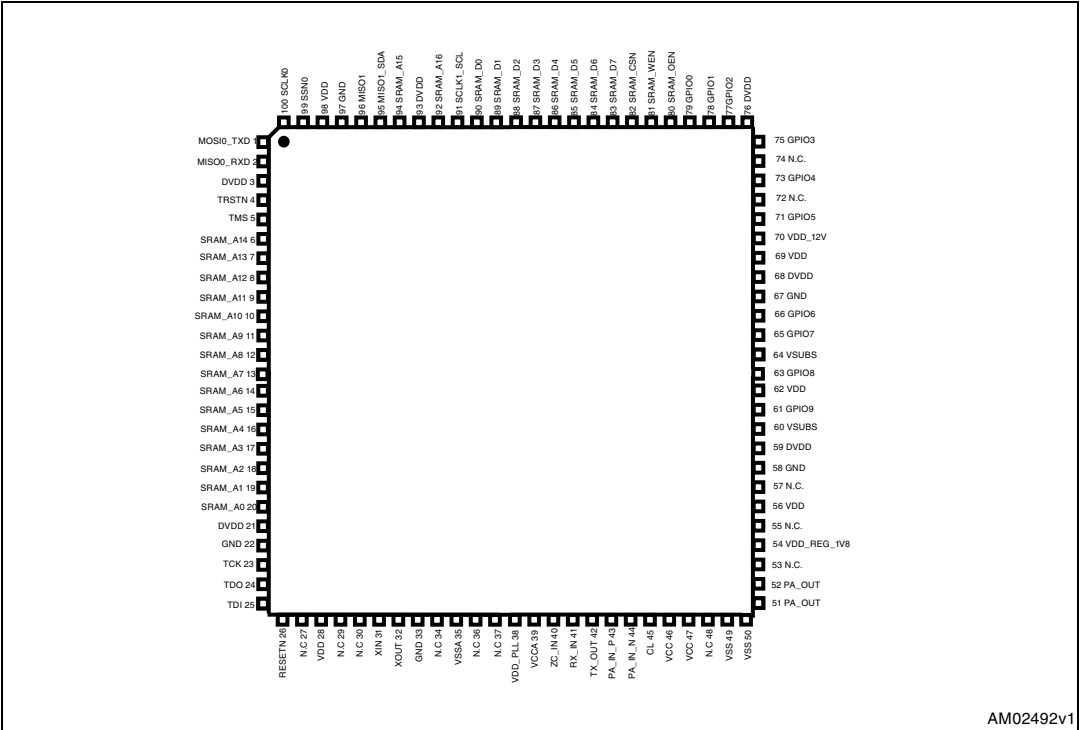
Figure 2. TQFP100 pin connection
