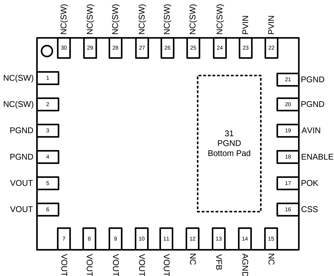
Figure 3: Pin Out Diagram (Top View)
