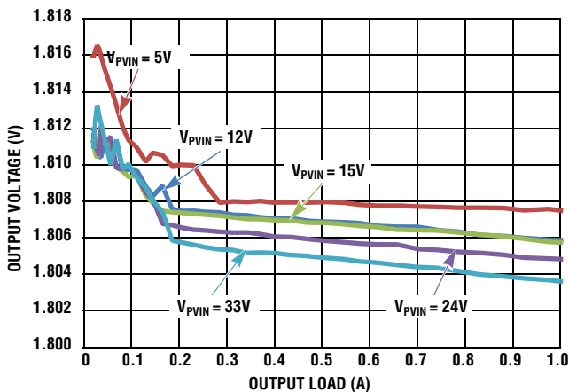
FIGURE 18. V_{OUT} REGULATION vs LOAD, PFM, V_{OUT} = 1.8\text{V}
