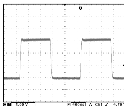
Figure 7 - IXDD408 Typical Waveform F=500KHz, CL=10000pF
