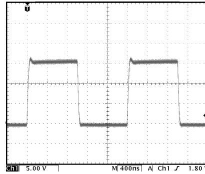
Figure 10 - IXDD414 Typical Waveform F=500KHz, CL=10000pF
