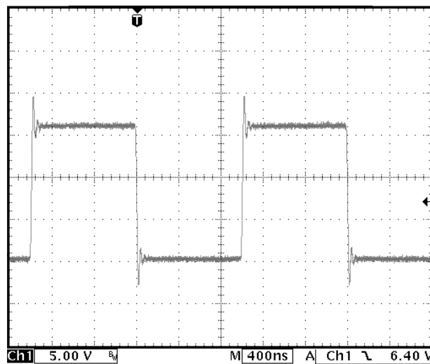
Figure 6 - IXDD404 Typical Output Waveform F=500KHz, CL=1800pF
