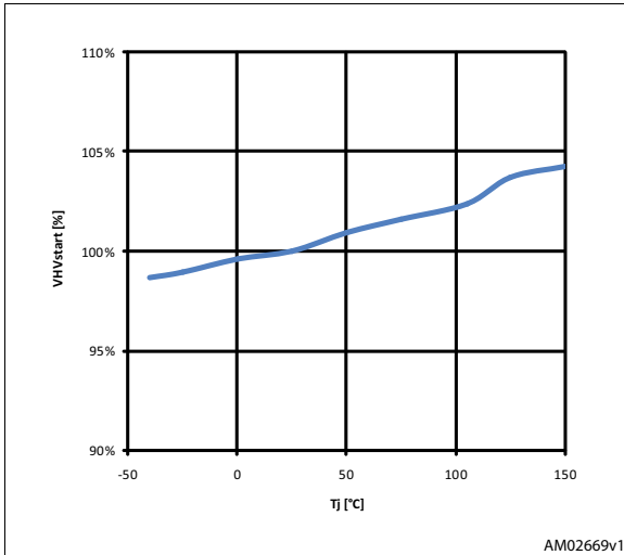
Figure 6. High-voltage generator start voltage vs. Tj
