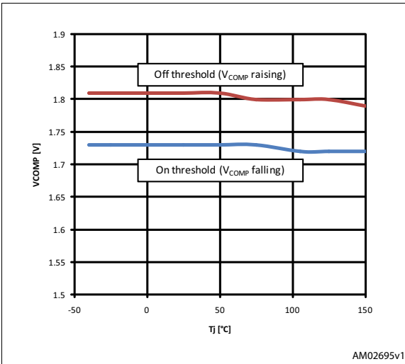
Figure 34. Line sensing threshold vs. Tj
