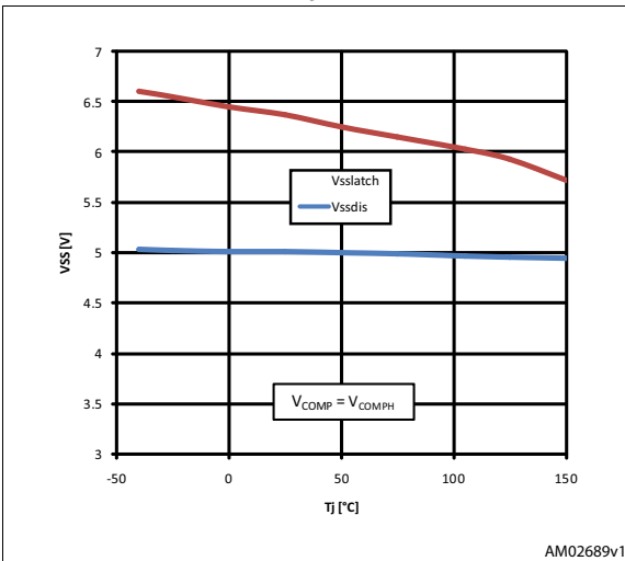
Figure 26. Soft-start disable and latch-off levels vs. Tj
