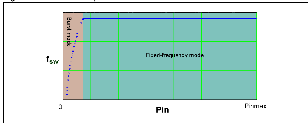
Figure 39. Multi-mode operation
