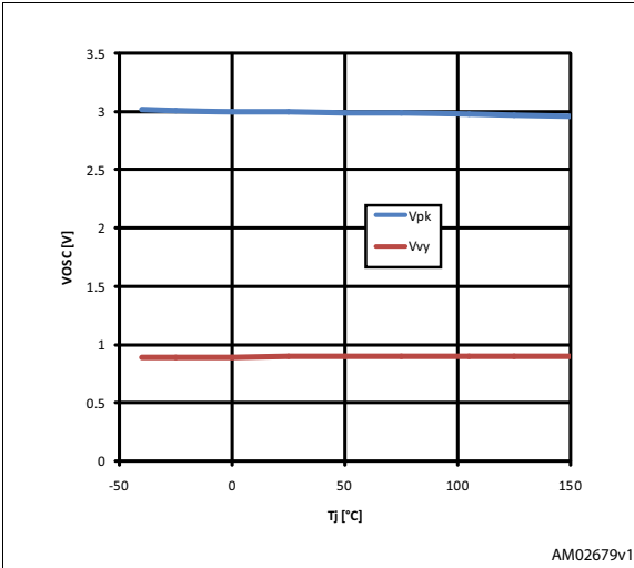
Figure 16. Oscillator ramp vs. Tj
