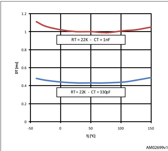
Figure 38. Dead time vs. R_T , C_T
