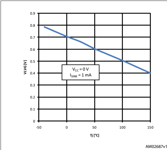
Figure 24. UVLO saturation vs. Tj
