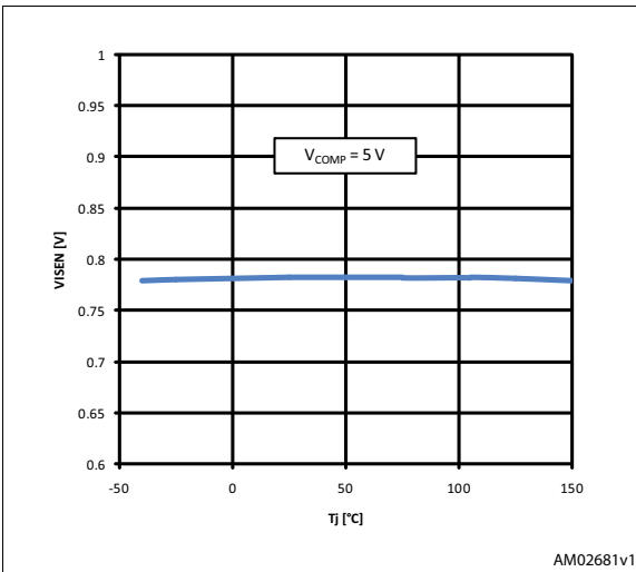
Figure 18. Current sense clamp vs. Tj
