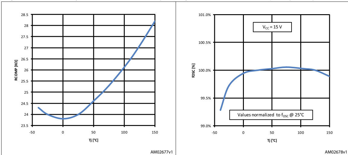
Figure 14. COMP dynamic resistance vs. T_j vs. Figure 15. Oscillator frequency vs. T_j
