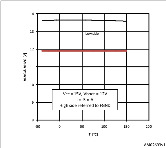
Figure 30. Gate-drives output high voltage vs. Tj
