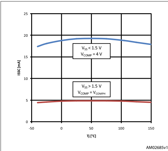
Figure 22. Soft-start charge current vs. Tj
