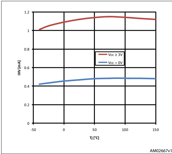
Figure 4. High-voltage generator ON-state sink current vs. Tj
