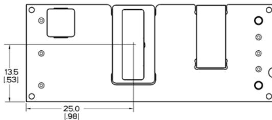
Figure 20. Pick and Place Location.
