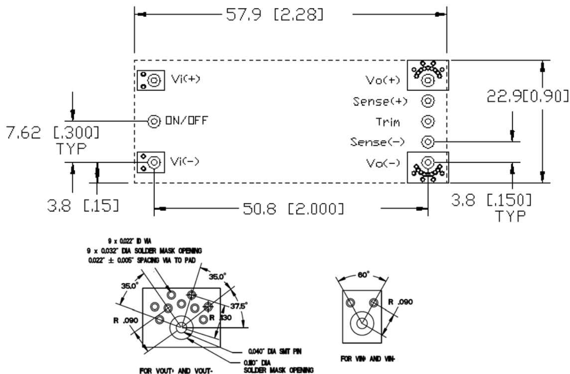
SMT Recommended Pad Layout (Component Side View)
