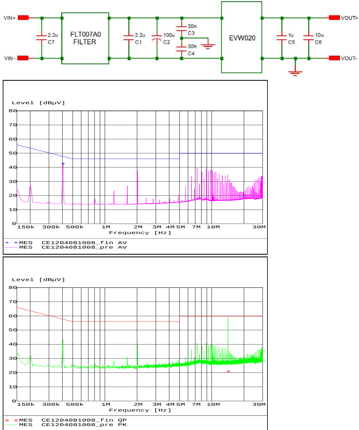
Figure 25. EMC Considerations
