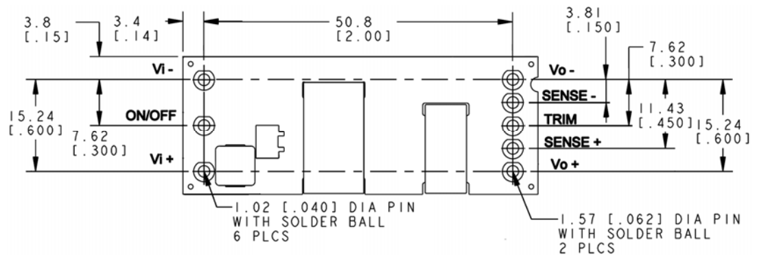
Bottom View
