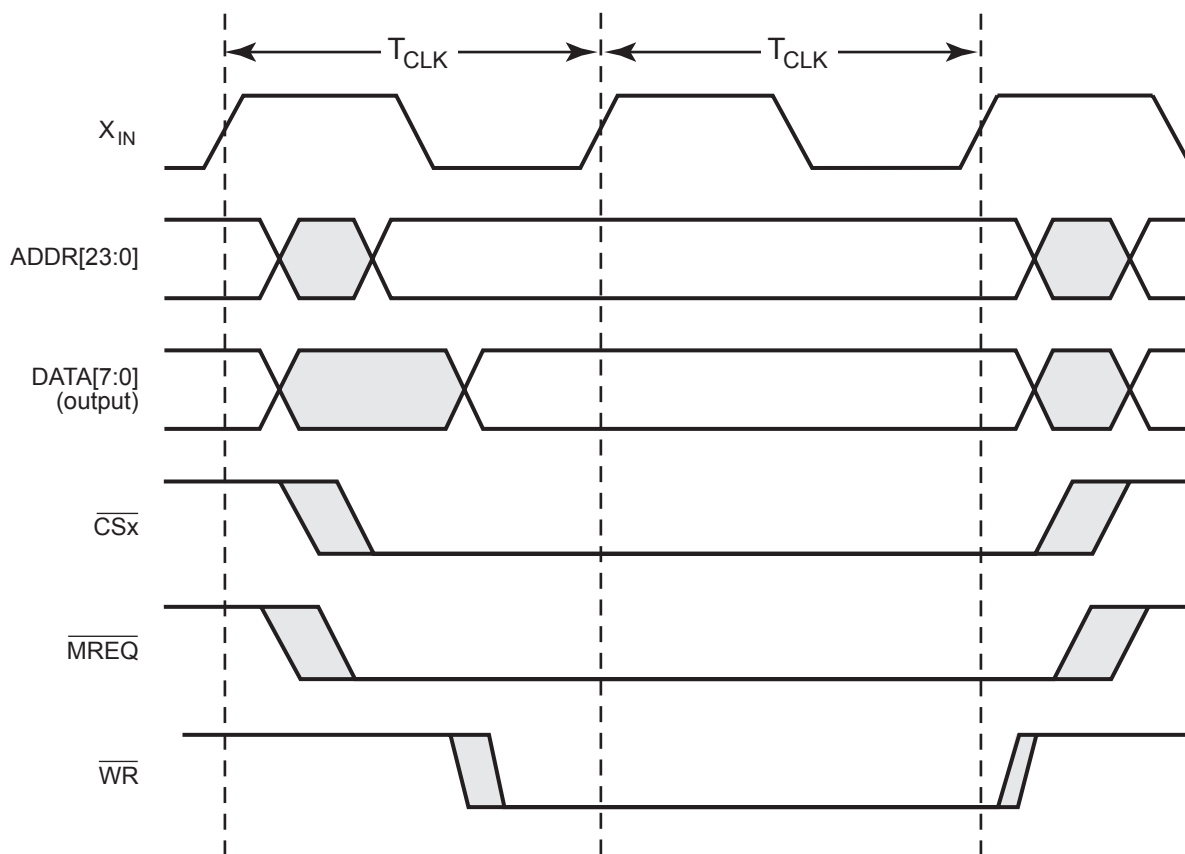
Figure 53. Wait State Timing for Write Operations
