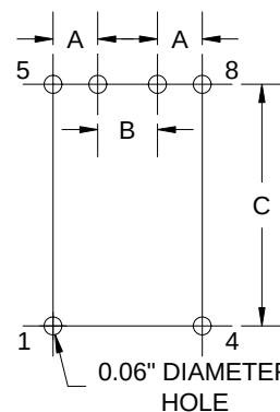
Board Layout
