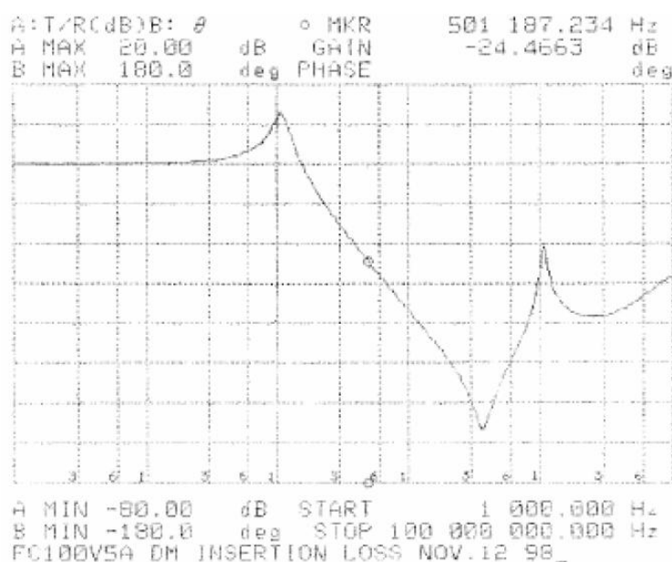
Figure 4. Differential Mode Attenuation Plot
