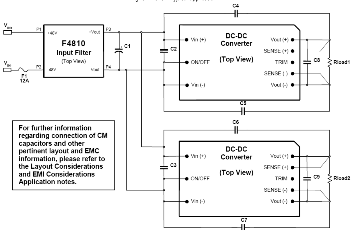
Fig. 5: F4810 – Typical application
