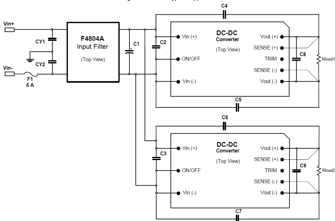
Fig. 5: F4804A - Typical Application
