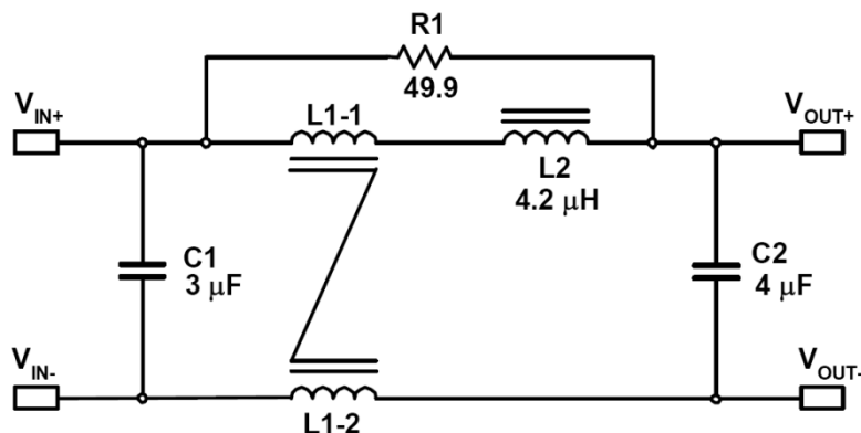
Fig. 1: Schematic diagram for F4810, F2410. The Capacitor values shown are for F4810; for F2410 C1=10 \mu\text{F} ; C2=13 \mu\text{F} .
