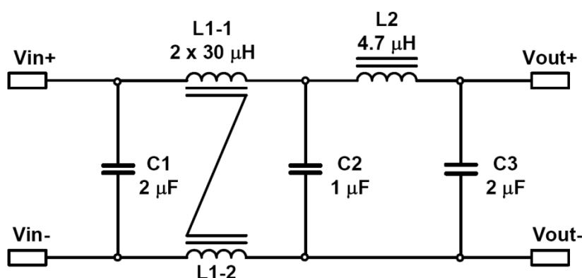
Fig. 1: Schematic Diagram.
