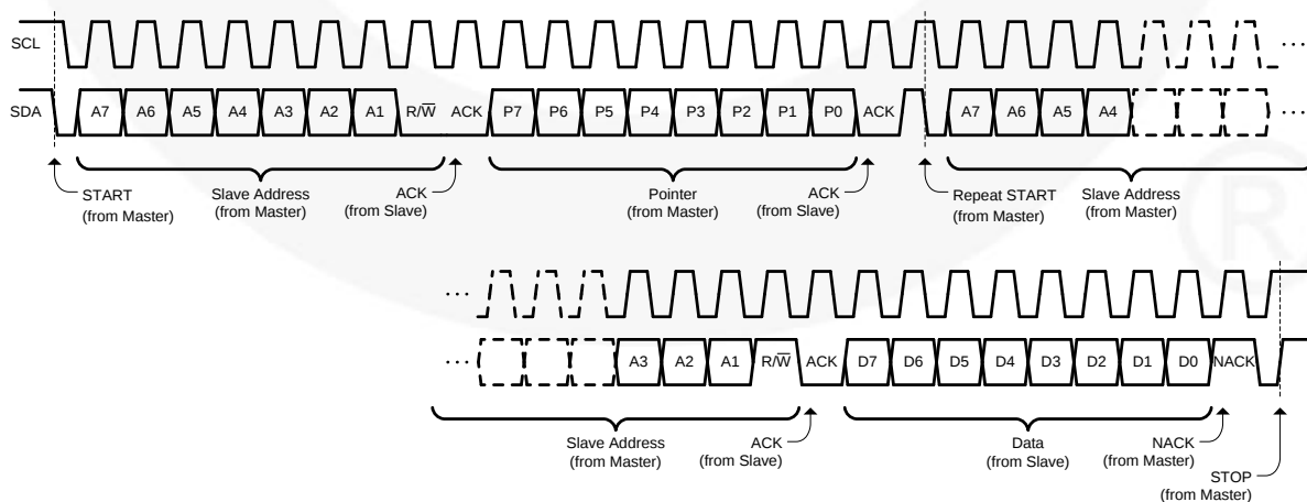
Figure 22. I²C Write Followed by Read
