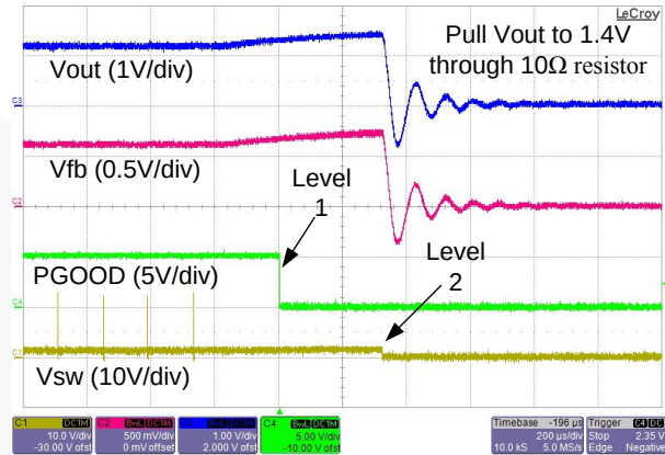
Figure 29. Over-Voltage Protection Level 1 and Level 2
