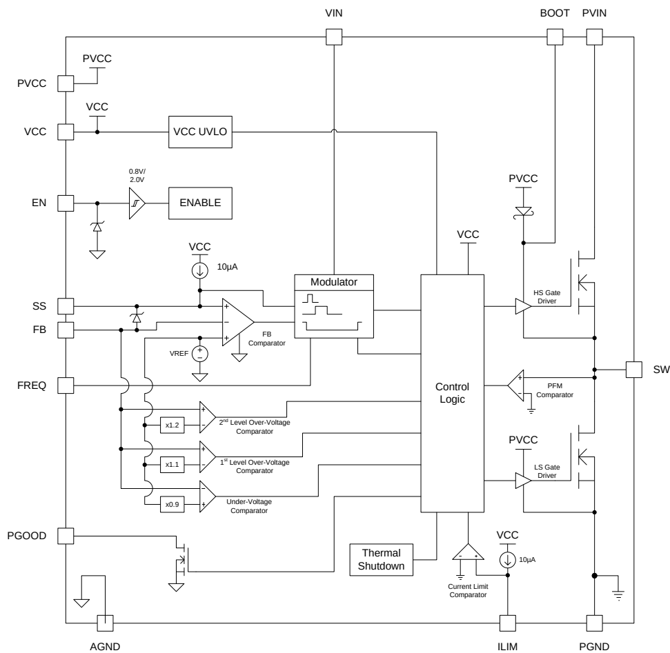
Figure 2. Block Diagram
