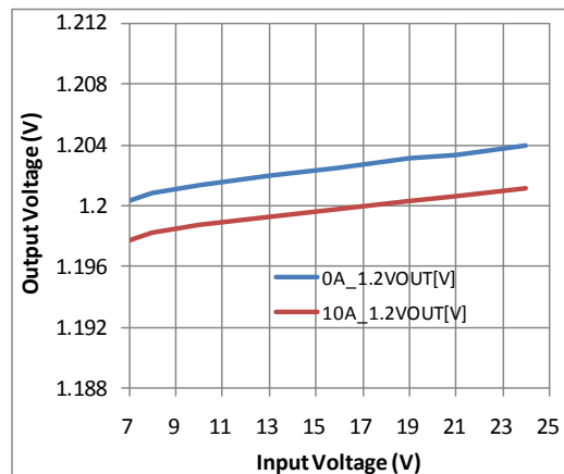
Figure 12. Line Regulation
