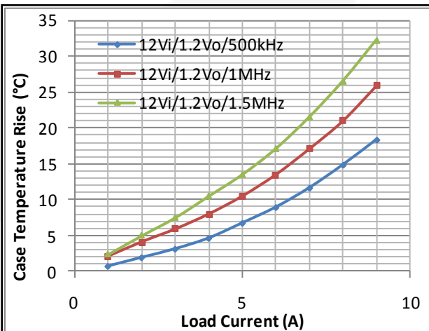
Figure 11. Case Temperature Rise vs. Load Current on 4 Layer PCB, 1 oz Copper, 7 cm x 7 cm
