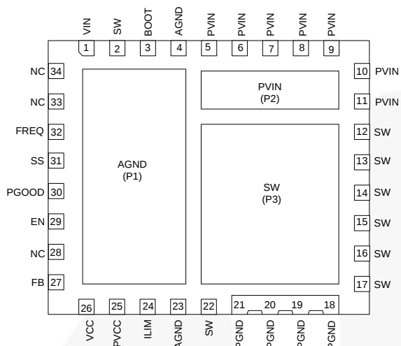
Figure 4. Pin Assignments, Bottom View
