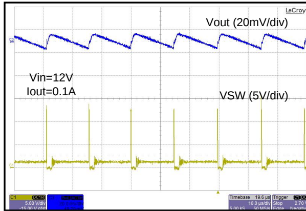
Figure 18. FAN23SV06 Static Output Ripple at Light Load
