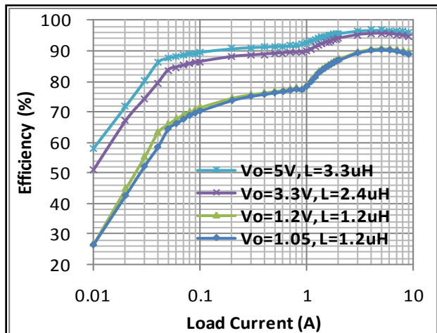
Figure 6. FAN23SV06 Efficiency vs. Load Current with V_{IN}=12\text{ V} and f_{SW}=500\text{ kHz}
