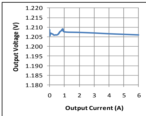
Figure 12. Load Regulation
