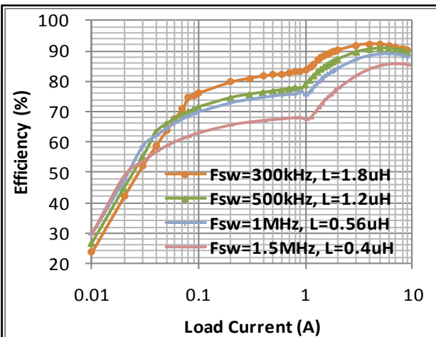
Figure 7. FAN23SV06 Efficiency vs. Load Current with V_{IN}=12\text{ V} and V_{OUT}=1.2\text{ V}
