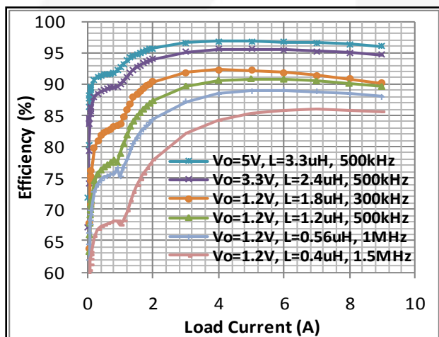
Figure 8. FAN23SV06 Efficiency vs. Load Current with V_{IN}=12\text{ V}
