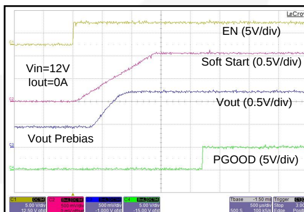
Figure 17. FAN23SV06 Startup Waveforms with Pre-Bias Voltage on Output
