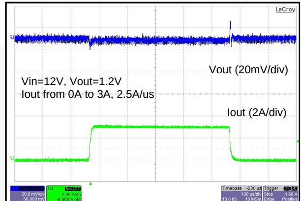
Figure 25. FAN23SV06P Load Transient from 0% to 50% Load Current
