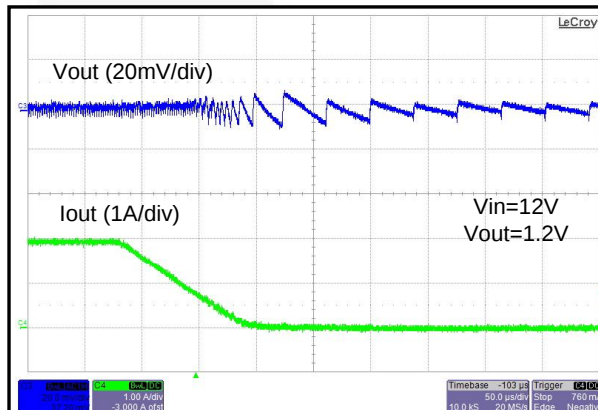
Figure 22. FAN23SV06 Operation as Load Changes from 2 A to 0 A
