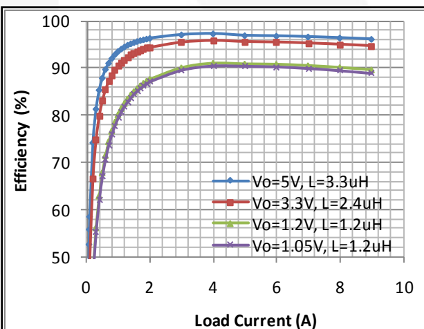
Figure 9. FAN23SV06P Efficiency vs. Load Current V_{IN}=12\text{ V} and f_{SW}=500\text{ kHz}
