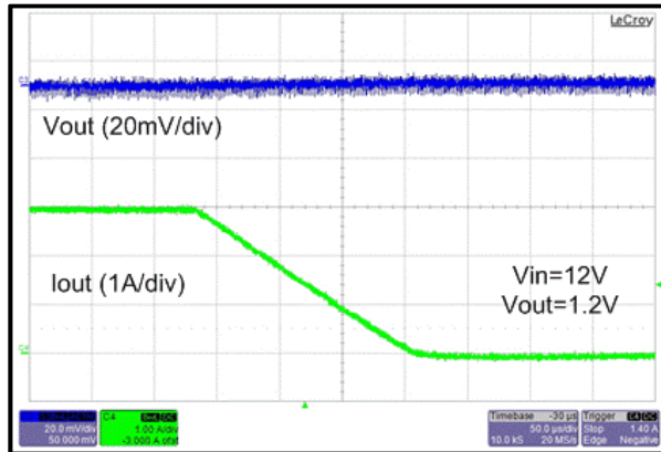
Figure 24. FAN23SV06P Operation as Load Changes from 3 A to 0 A
