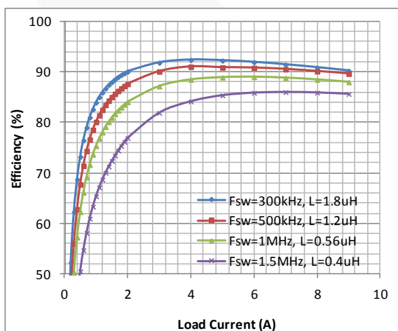
Figure 10. FAN23SV06P Efficiency vs. Load Current with V_{IN}=12\text{ V} and V_{OUT}=1.2\text{ V}
