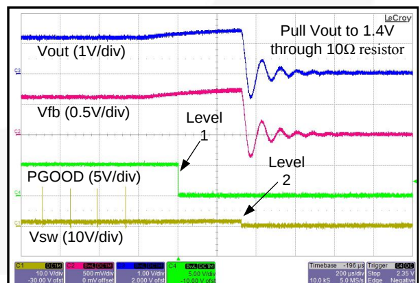
Figure 29. Over-Voltage Protection Level 1 and 2
