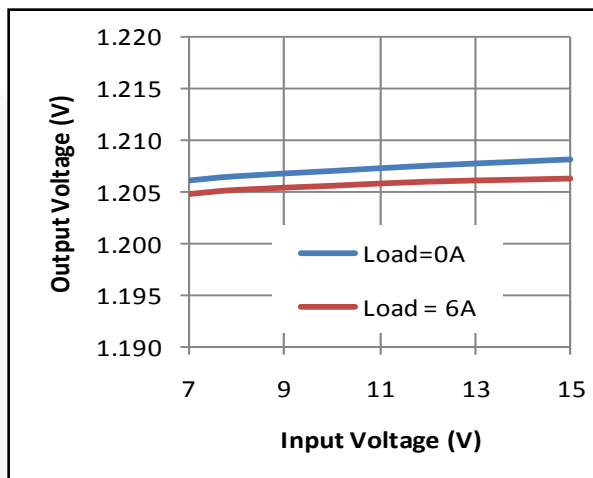
Figure 13. Line Regulation
