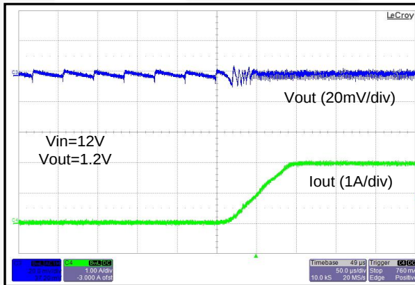
Figure 21. FAN23SV06 Operation as Load Changes from 0 A to 2 A
