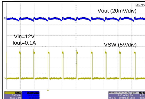
Figure 20. FAN23SV06P Static Output Ripple with No Load
