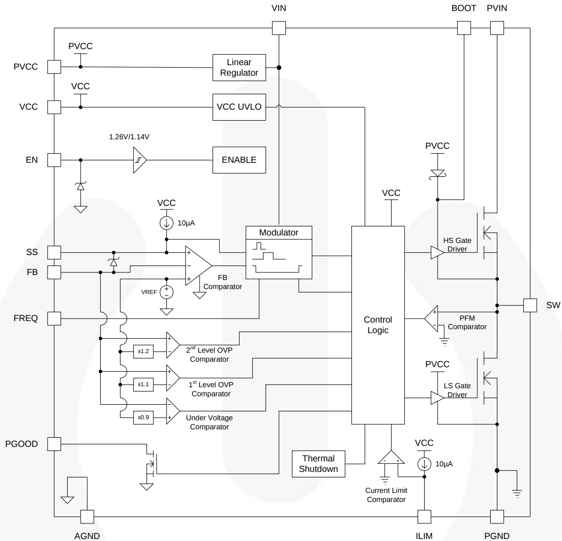
Figure 3. Block Diagram
