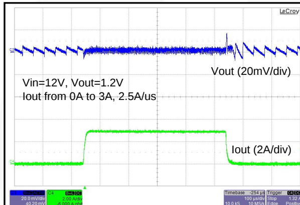
Figure 26. FAN23SV06 Load Transient from 0% to 50% Load Current
