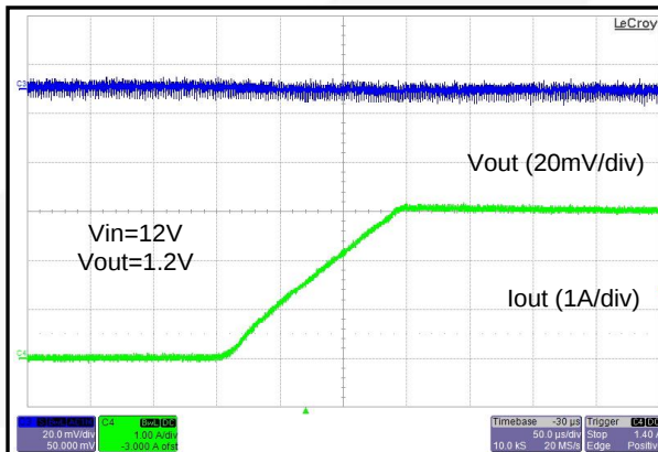
Figure 23. FAN23SV06P Operation as Load Changes from 0 A to 3 A
