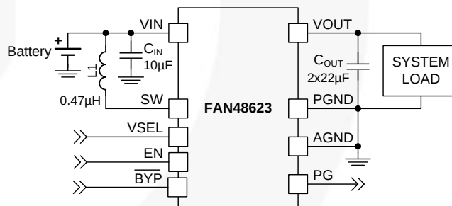
Figure 1. Typical Application
