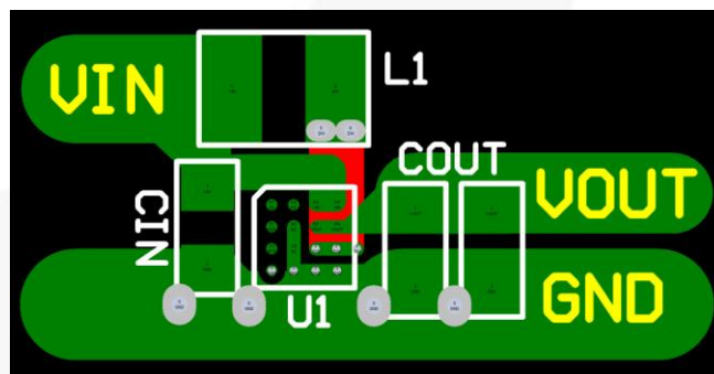
Figure 41. Layout Recommendation
