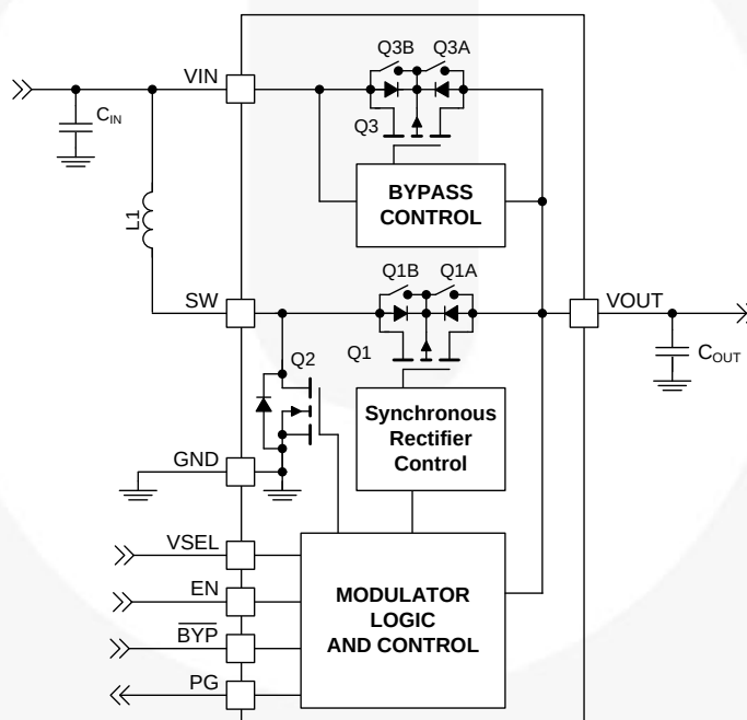
Figure 2. Block Diagram
