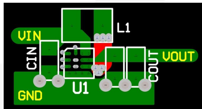
Figure 29. Layout Recommendation
