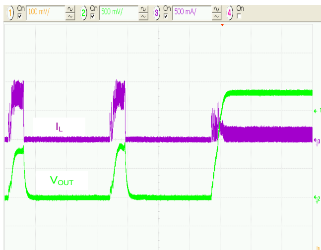
Figure 17. Overload Recovery to Light Load, 100µs/div.
