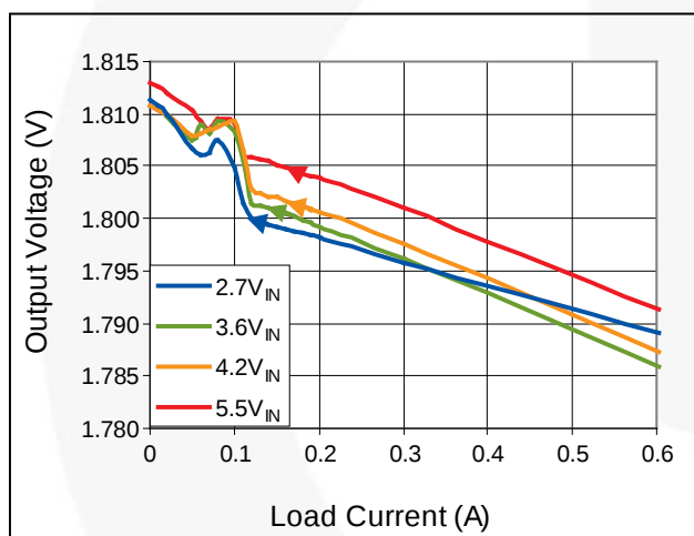
Figure 6. Voltage Regulation
