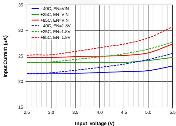
Figure 14. Quiescent Current vs. Input Voltage and Temperature, Auto Mode; EN = V_{IN} Solid, Dotted for EN = 1.8 V (-40°C, +25°C, +85°C)
