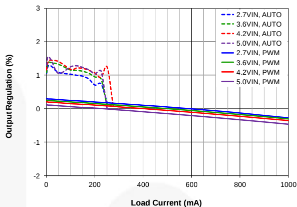
Figure 11. \Delta V_{OUT} (%) vs. Load Current and Input Voltage, V_{OUT} = 1.23 V, Normalized to 3.6 V_{IN} , 500 mA Load, FPWM, Dotted for Auto Mode
