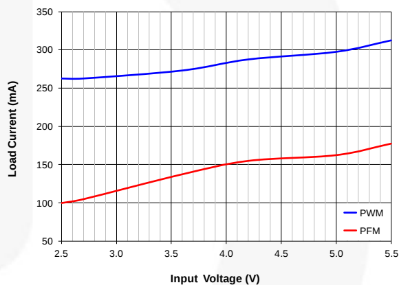
Figure 13. PFM / PWM Boundary vs. Input Voltage, V_{OUT} = 1.23 V
