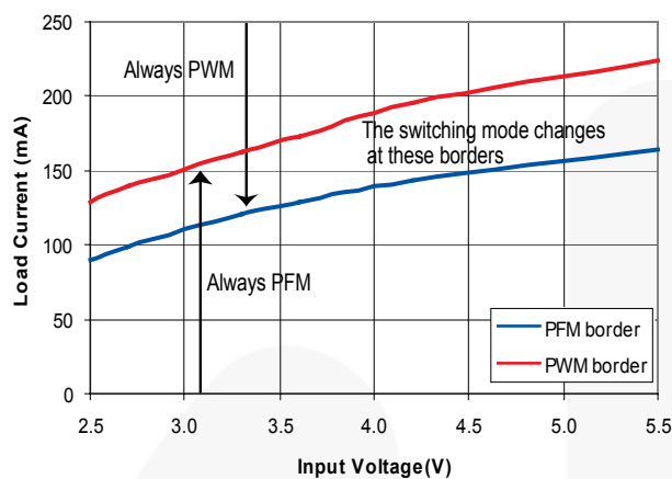
Figure 17. 1.233V OUT PFM / PWM Boundaries
