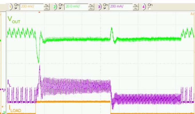
Figure 25. Load Transient 50 to 250mA, 2.5V_{IN}
