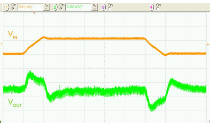
Figure 21. Line Transient 3.3\text{ V}_{IN} to 3.9\text{ V}_{IN} , 250\text{ mA} Load, 10\mu\text{s/div.}
