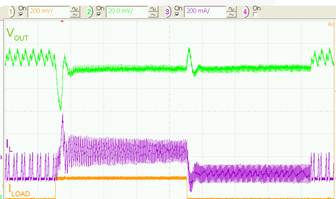
Figure 25. Load Transient 50 to 250\text{ mA} , 2.5\text{ V}_{IN}
