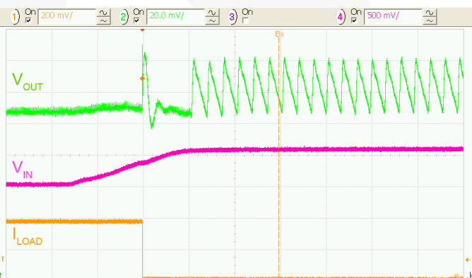
Figure 23. Combined Line/Load Transient 3.3 to 3.9\text{ V}_{IN} Combined with 400\text{ mA} to 40\text{ mA} Load Transient
