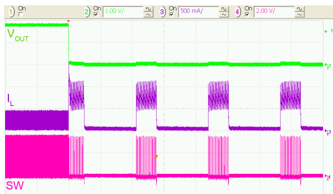
Figure 33. Metallic Short Applied at V_{OUT} , 50 \mu\text{s}/\text{div} .
