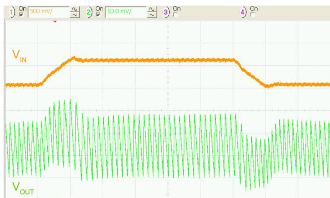
Figure 20. Line Transient 3.3\text{ V}_{IN} to 3.9\text{ V}_{IN} , 50\text{ mA} Load, 10\mu\text{s/div.}
