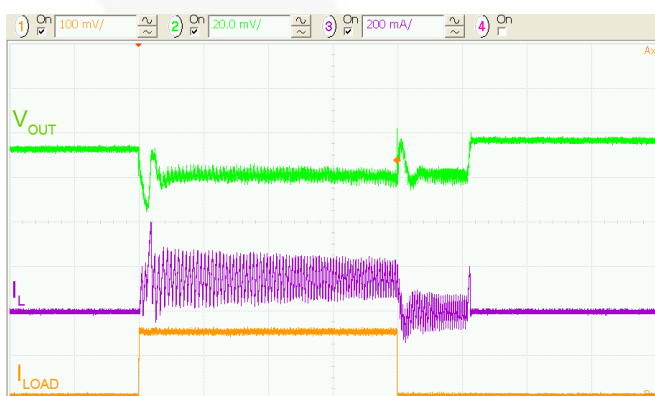
Figure 24. Load Transient 0 to 150\text{ mA} , 2.5\text{ V}_{IN}
