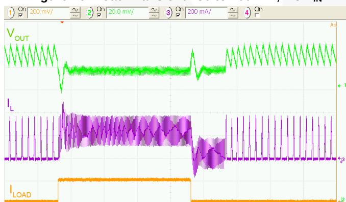
Figure 28. Load Transient 50 to 250 mA, 3.6\text{ V}_{IN}
