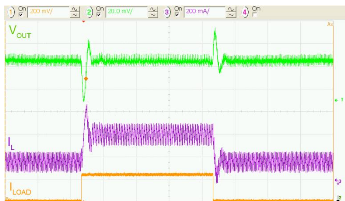
Figure 26. Load Transient 150 to 400 mA, 2.5\text{ V}_{IN}
