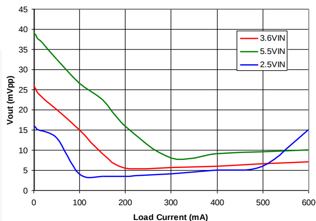
Figure 12. 1.82 V OUT Peak-to-Peak Output Voltage Ripple
