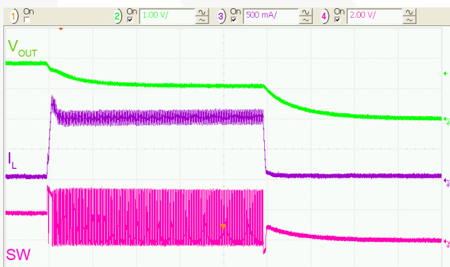
Figure 36. Over-Current Fault Response, R_{LOAD} = 1 \Omega
