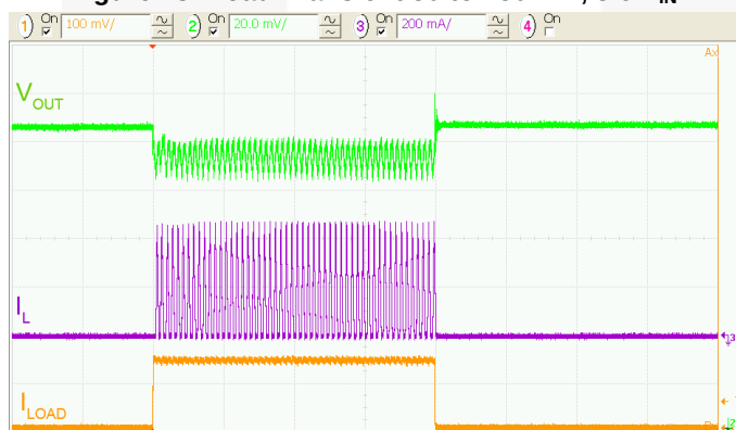
Figure 30. Load Transient 0 to 150 mA, 4.5\text{ V}_{IN}
