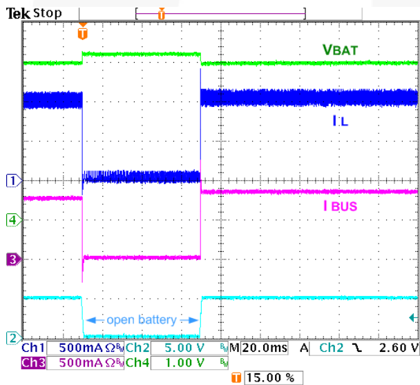
Figure 15. Battery Removal / Insertion During Charging, V_{BAT}=3.9 V, I_{OCHARGE}=1,050 mA, No I_{INLIM} , TE=0
