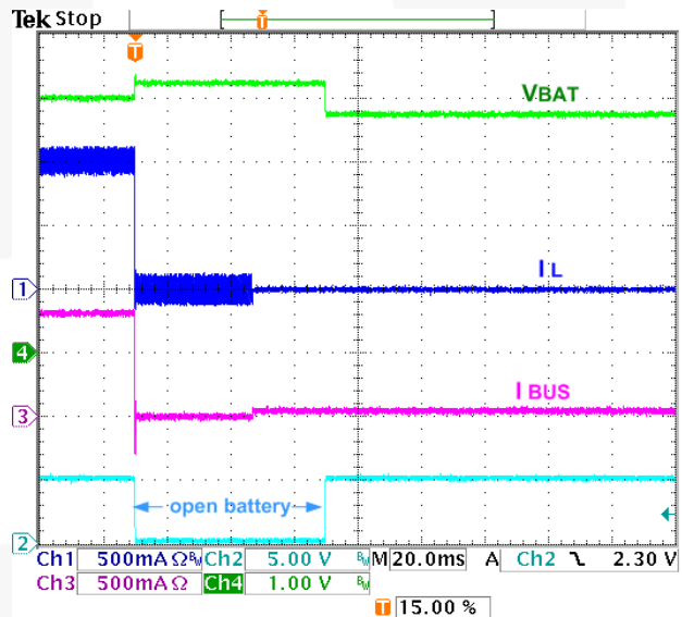
Figure 16. Battery Removal / Insertion During Charging, V_{BAT}=3.9 V, I_{OCHARGE}=1,050 mA, No I_{INLIM} , TE=1
