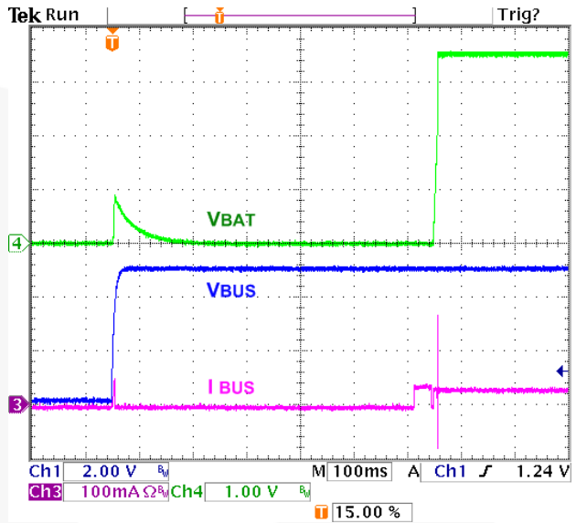
Figure 18. No Battery at V_{\text{BUS}} Power-up; FAN54012
