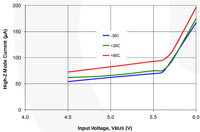
Figure 19. V_{\text{BUS}} Current in High-Impedance Mode with Battery Open
