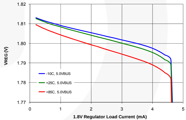
Figure 20. V_{\text{REG}} 1.8 V Output Regulation
