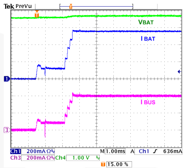
Figure 14. Charger Startup with HZ_MODE Bit Reset, I_{INLIM}=500 mA, I_{OCHARGE}=1,050 mA, OREG=4.2 V, V_{BAT}=3.6 V
