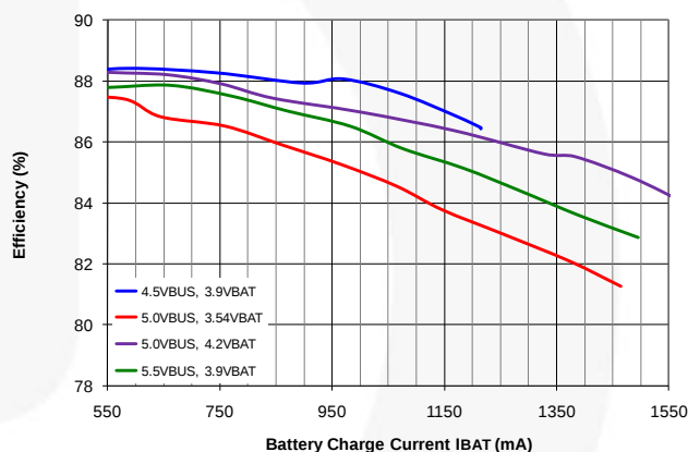
Figure 10. Efficiency vs. Charging Current, I_{\text{BUSLIM}}=\text{No Limit}
