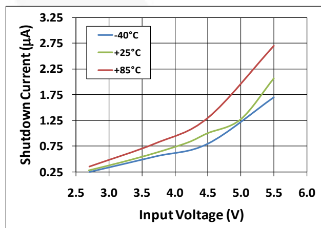
Figure 15. Shutdown Current vs. Input Voltage vs. Temperature
