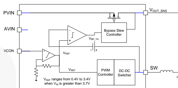
Figure 55. Enabling Bypass Transistor Circuit
