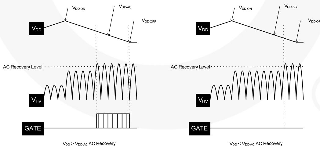
Figure 7. V_{DD-AC} and AC Recovery
