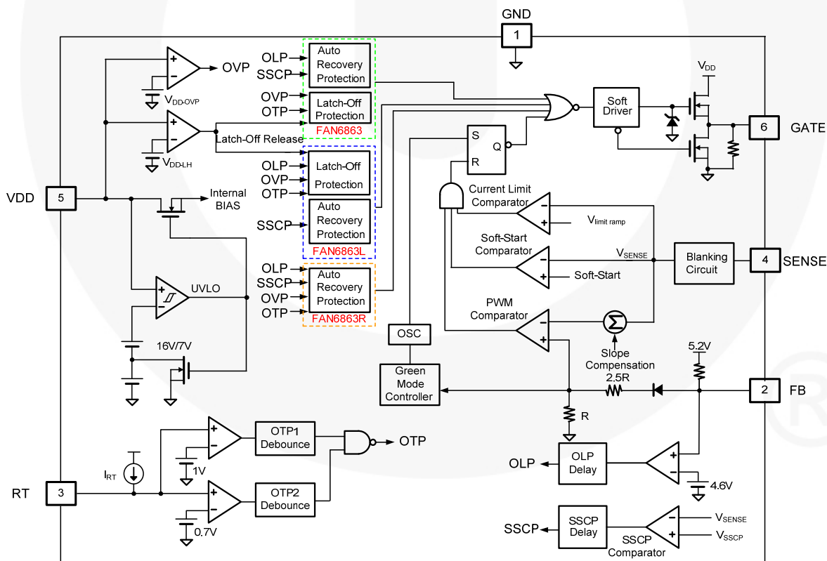
Figure 2. Block Diagram
