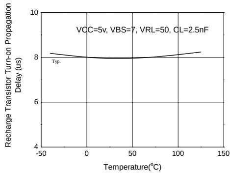
Figure 12. Recharge FET Turn-on Delay time
