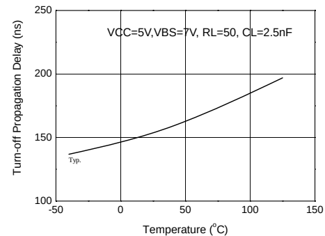
Figure 6b. Turn-Off Propagation Delay Time vs Temperature
