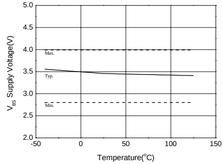
Figure 10b. VBS Under Voltage Threshold(-) vs Temperature
