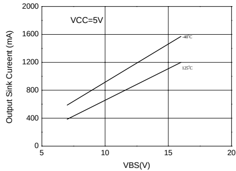
Figure5a. Output Sink Current vs VBS Supply
