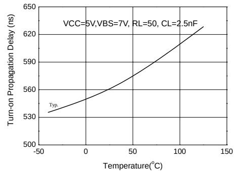
Figure 6a. Turn-On Propagation Delay Time vs Temperature
