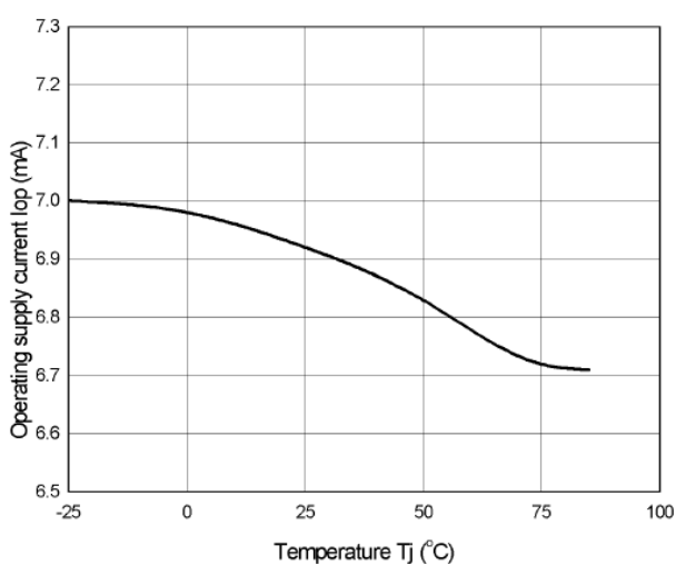
Figure 9. Temperature vs. Operating Supply Current
