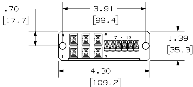
FRONT VIEW SHOWN W/O DUSTCAPS
