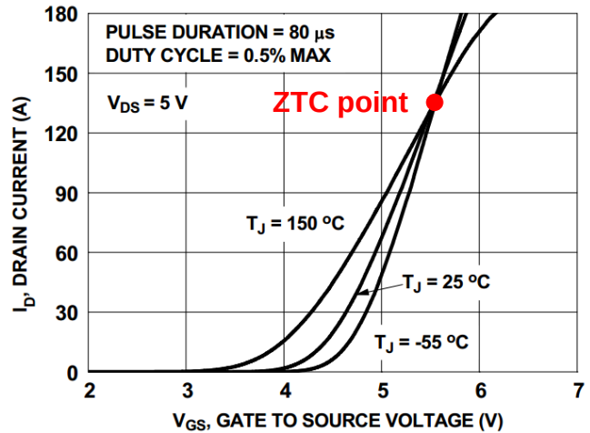
Figure 9. Transfer Characteristics
