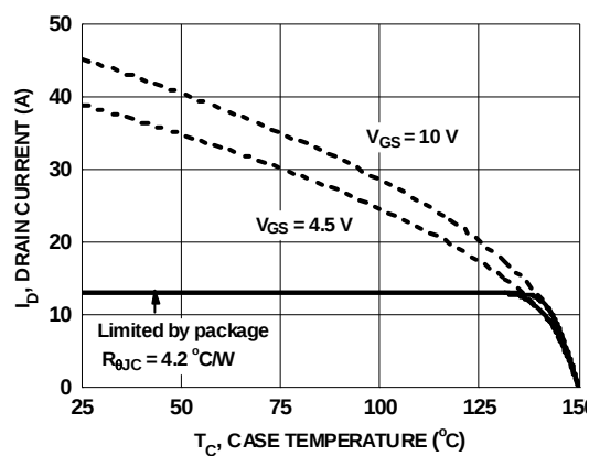
Figure 23. Maximum Continuous Drain Current vs. Case Temperature
