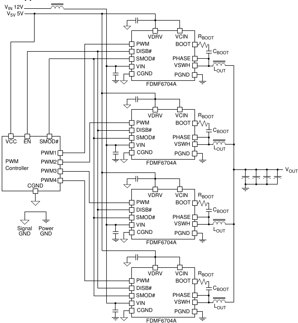
Figure 23. Typical Application
