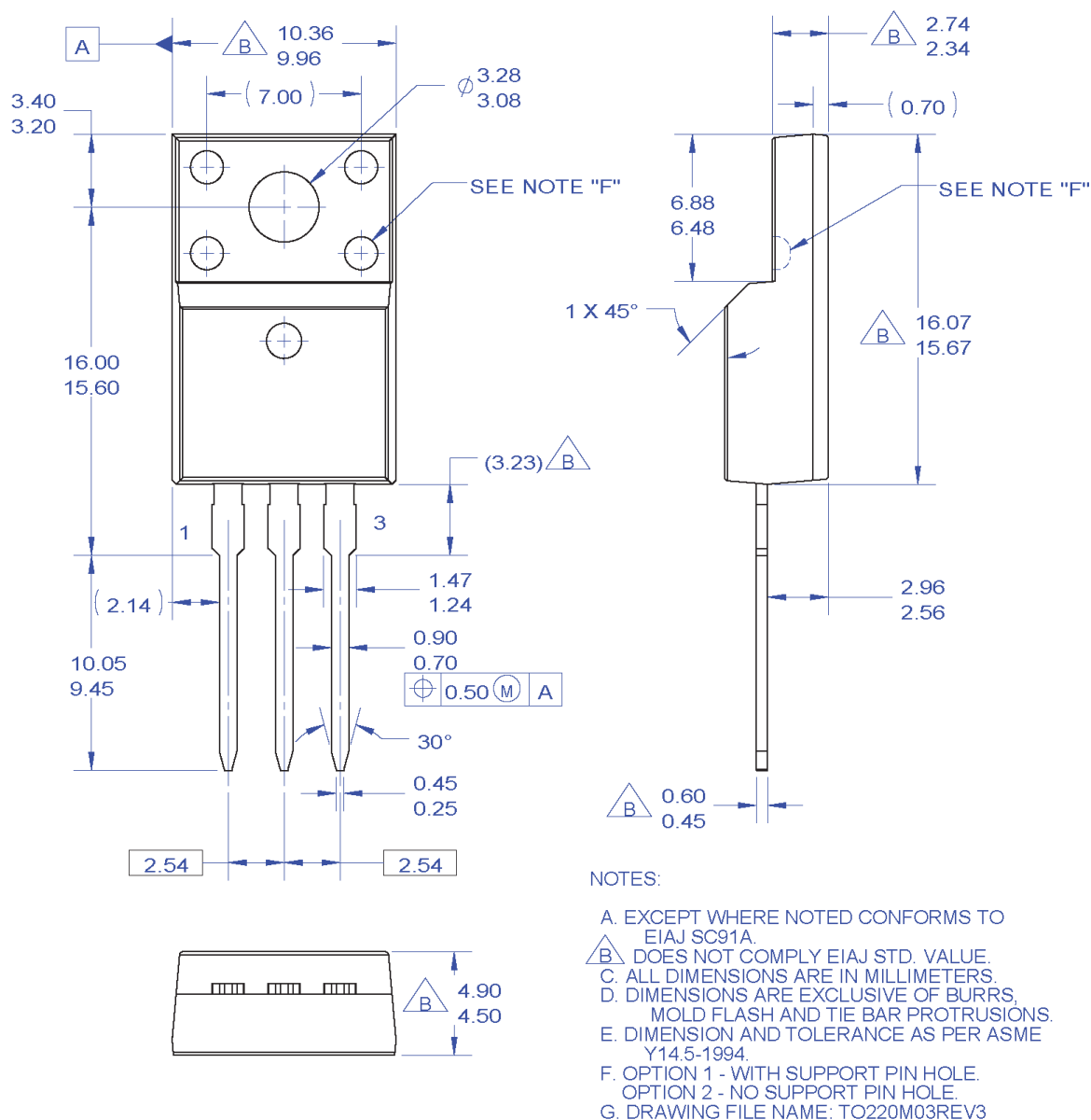
Figure 20. TO220, Molded, 3-Lead, Full Pack, EIAJ SC91, Straight Lead
