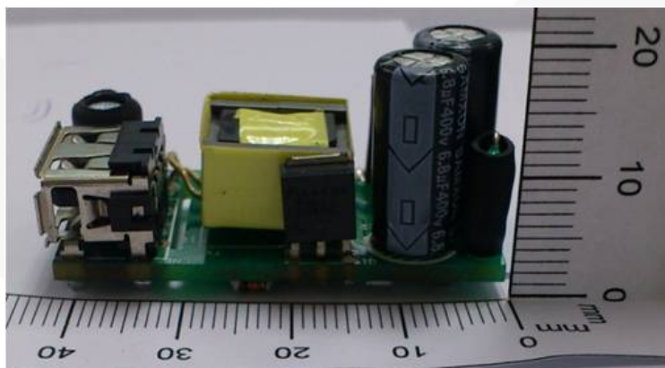
Figure 3. Photograph (32.4 (L) x 21 mm²(H)) Side-View
