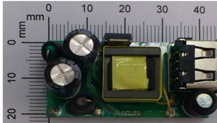
Figure 1. Photograph (32.4x 26 mm²) Top-View
