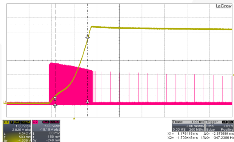
Figure 12. 90 V AC / 60 Hz, C1 [V O ], C2 [V GS ] at No Load
