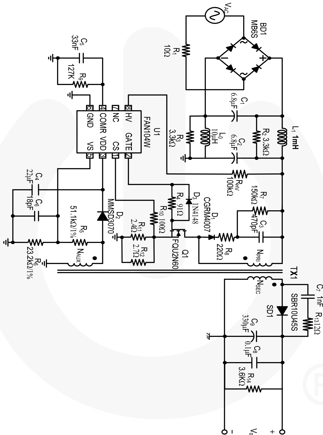
Figure 6. Evaluation Board Schematic
