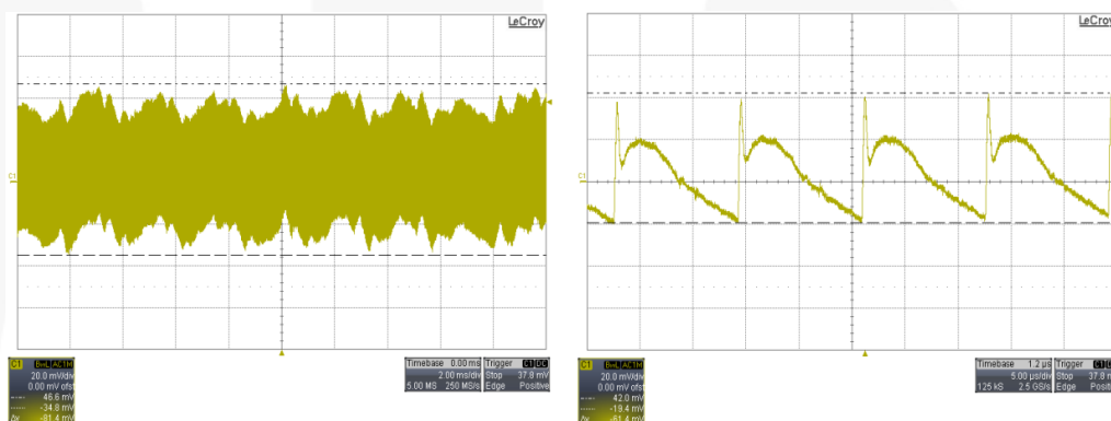
Figure 17. 90 V AC / 60 Hz, C1 [Vo] at Maximum Load
