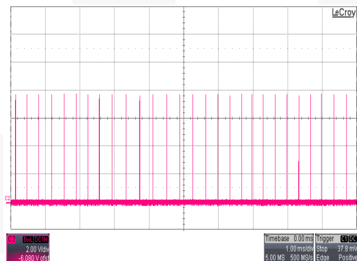
Figure 8. 90 V AC / 60 Hz, C2 [V cs ] at No Load
