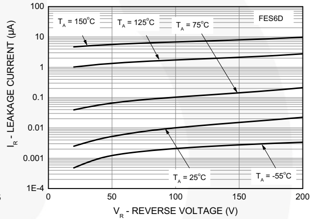
Fig 4. Typical Reverse Characteristics for FES6D
