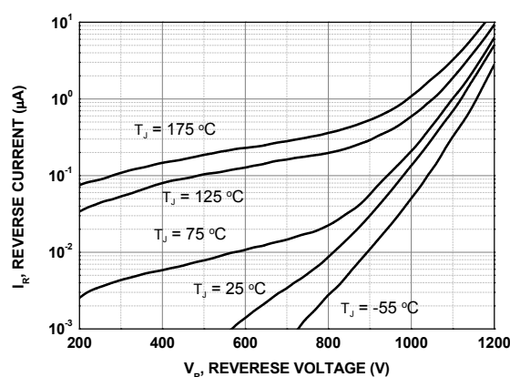
Figure 2. Reverse Characteristics
