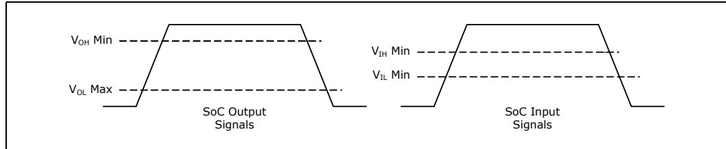
Figure 33-20. High and Low Signal Voltage Diagram - Single-Ended
