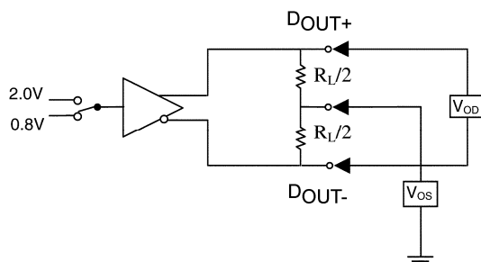
Figure 3. Differential Driver DC Test Circuit
