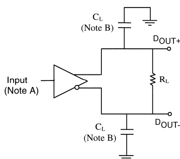
Figure 4. Differential Driver Propagation Delay and Transition Time Test Circuit
