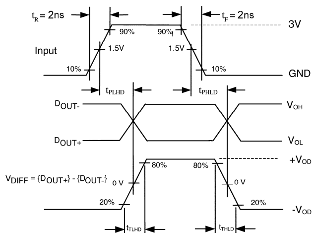
Figure 5. AC Waveforms
