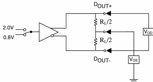
Figure 4. Differential Driver DC Test Circuit
