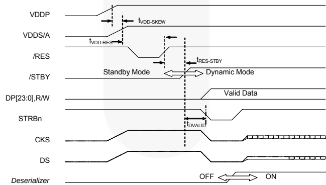
Figure 18. Power-Up Timing
