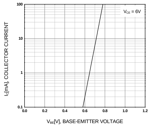
Figure 2. Transfer Characteristic
